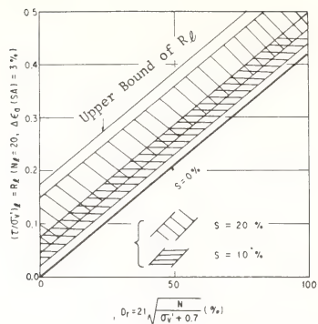
Fig. 29 D_r - R_L Relationship Based on Fig. 28
